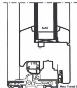
Seuil aluminium Maco Transit 20
