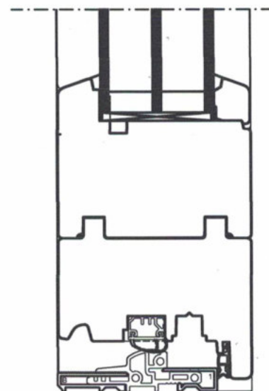
Seuil aluminium Maco Transit 20
