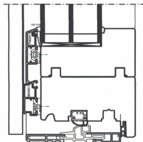
Seuil aluminium Maco Transit 20
