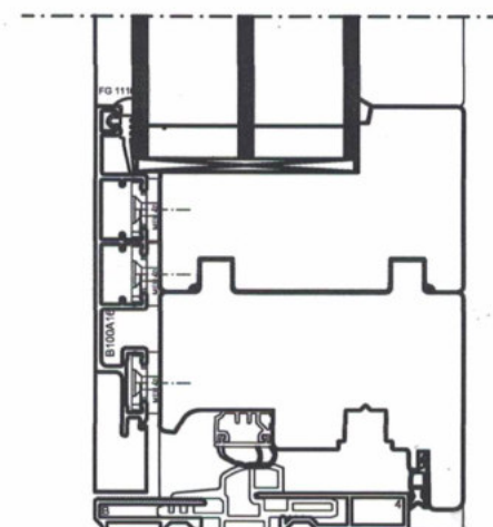
Seuil aluminium Maco Transit 20
